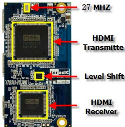
Figure 2.1 HDMI transmitter and receiver on the front of the HDMI board
