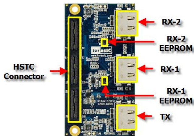
Figure 2.2 On the back of the HDMI board with HSTC connector and HDMI ports
