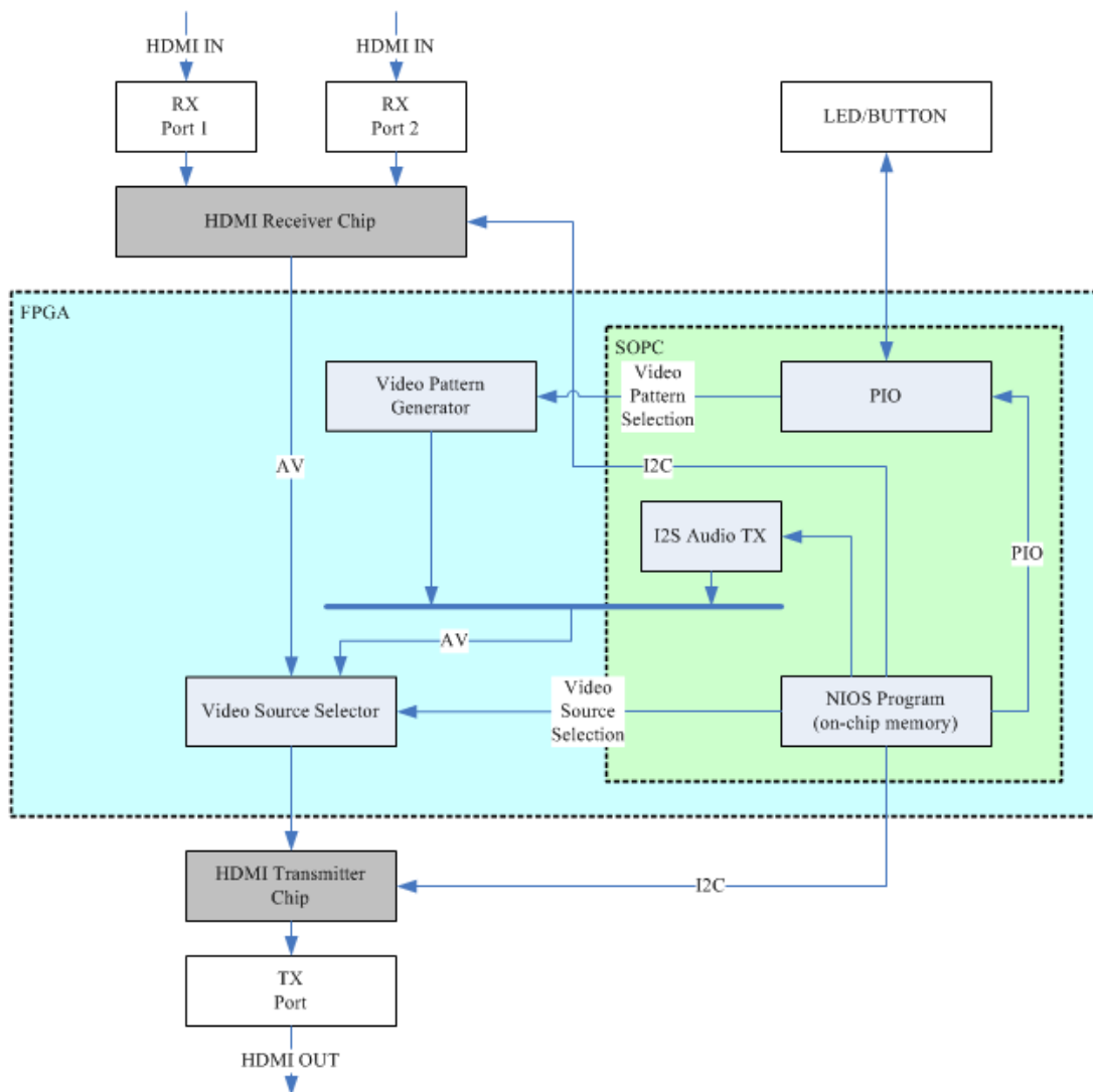
Figure 4.1. System Function Block Diagram
