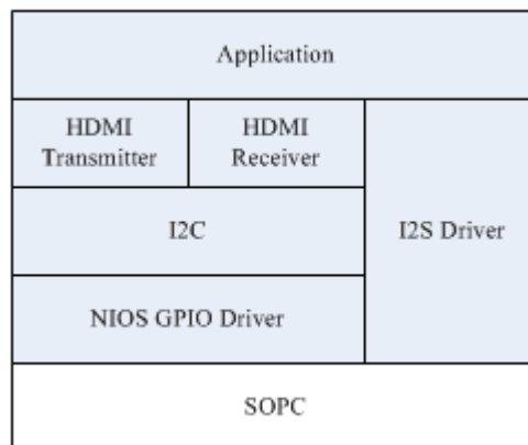
Figure 4.2 Software Stack
