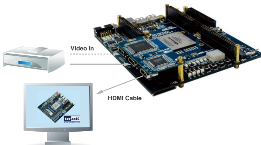
Figure 3.2 HDMI Loopback Demonstration Setup
