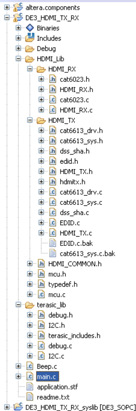
Figure 4.3 NIOS Program File List
