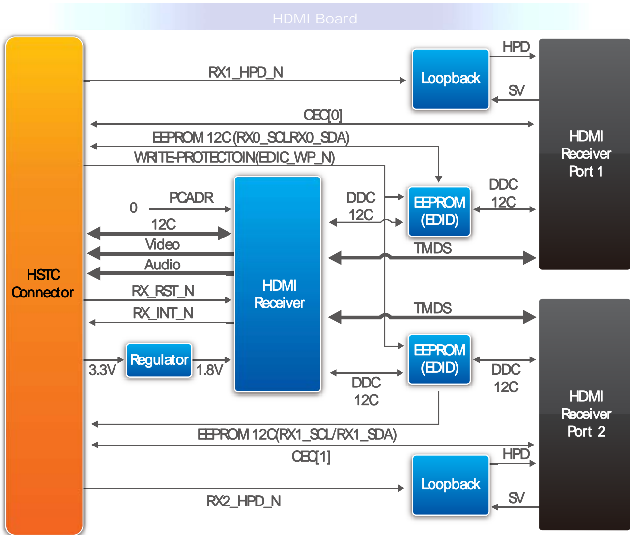
Figure 2.4 The block diagram of HDMI signal receiving
